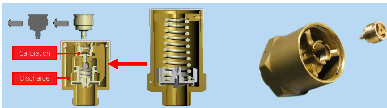
PV Safety valve with separate functions : calibration function and discharge
